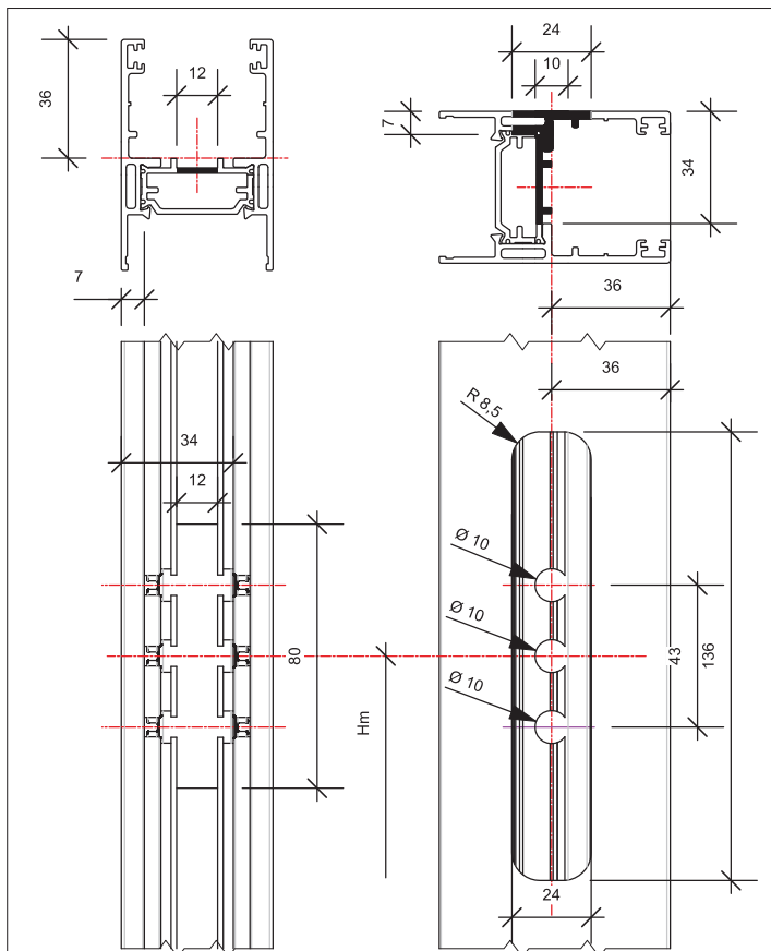
Maniglia con chiusura multipunto Handle with multi-point closure
