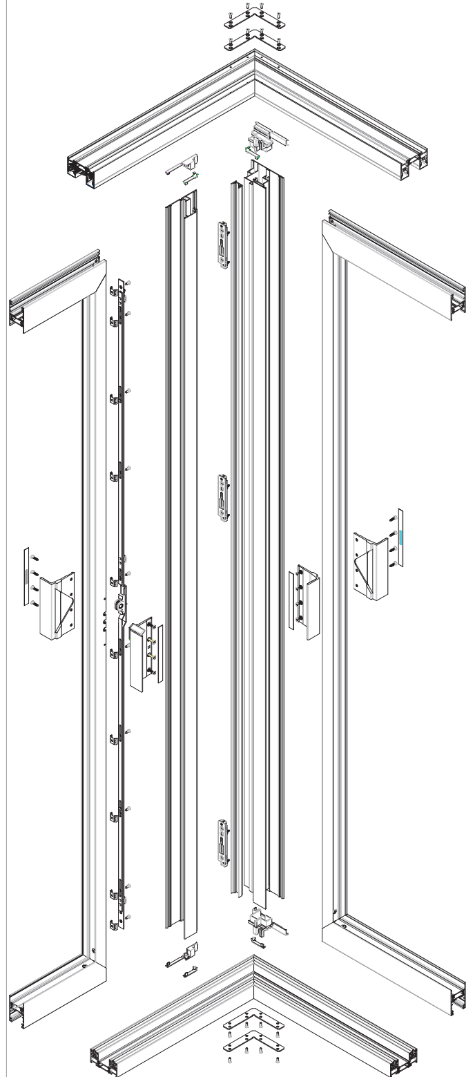
Detail of corner assembly doors
