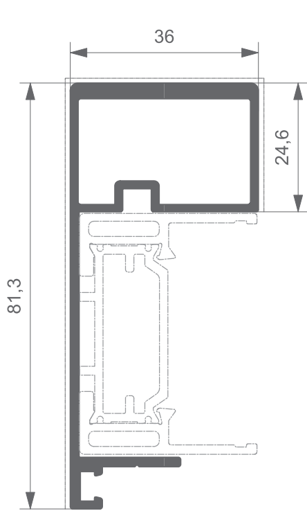
SX12.301 kg/ml 1,204 --- mm. 124,0
